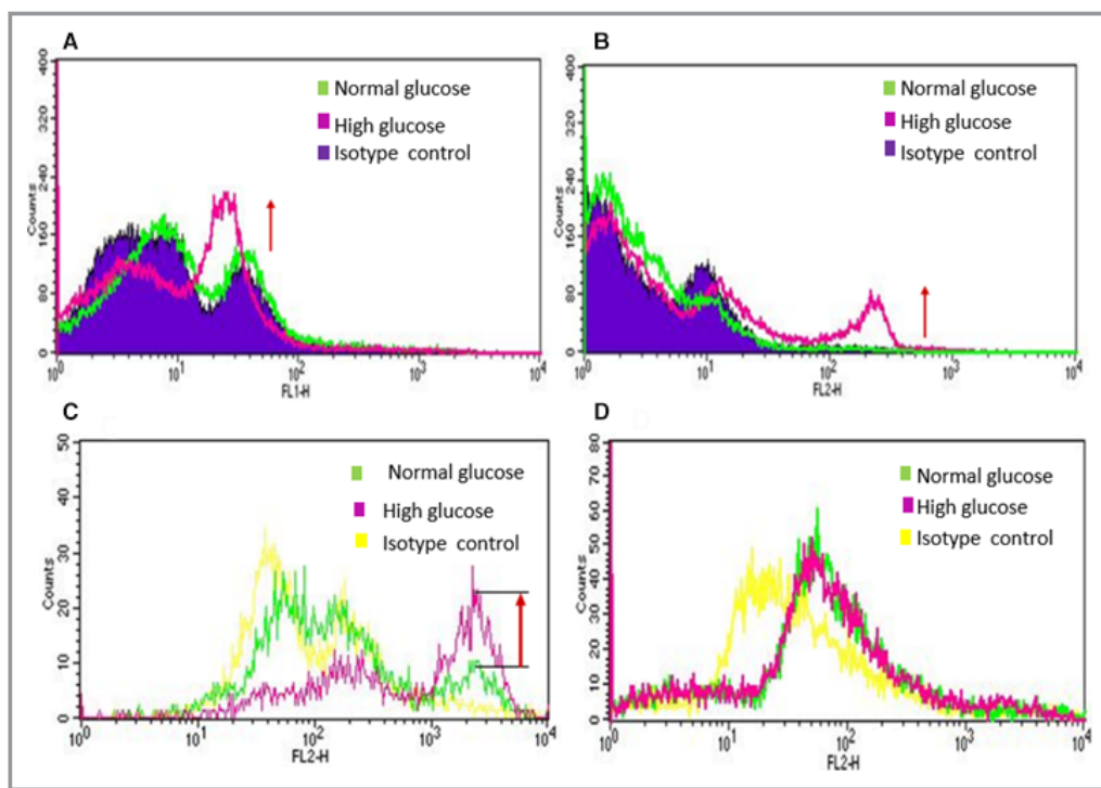
Figure 1. Fluorescence activated cell sorter (FACS) analysis of EPCs (CD34 + ) and HUVECs exposed to normal glucose (NG) and high glucose (HG): Human EPCs (CD34 + ) were exposed to NG (5.5 mmol/L) and HG (20 mmol/L) for 48 hours followed by FACS Analysis. A, Annexin V stained cells and B, Propidium iodide stained EPCs (CD34 + ) demonstrated significant degree of apoptosis takes place within 48 hours of high glucose exposure. To compare effect of NG and HG on endothelial progenitor and mature endothelial cells, C, human EPCs (CD34 + ) and D, HUVECs were exposed to NG and HG for 48 hours and 10 days, respectively, and cells were stained with propidium iodide. EPCs (CD34 + ) showed increased apoptosis by 48 hours of high glucose exposure. However, HUVECs did not show any apoptotic change even after 10 days of HG exposure compared to NG exposed cells. These data demonstrate that EPCs are more susceptible to HG mediated injury compared to mature endothelial cells (HUVECs).
