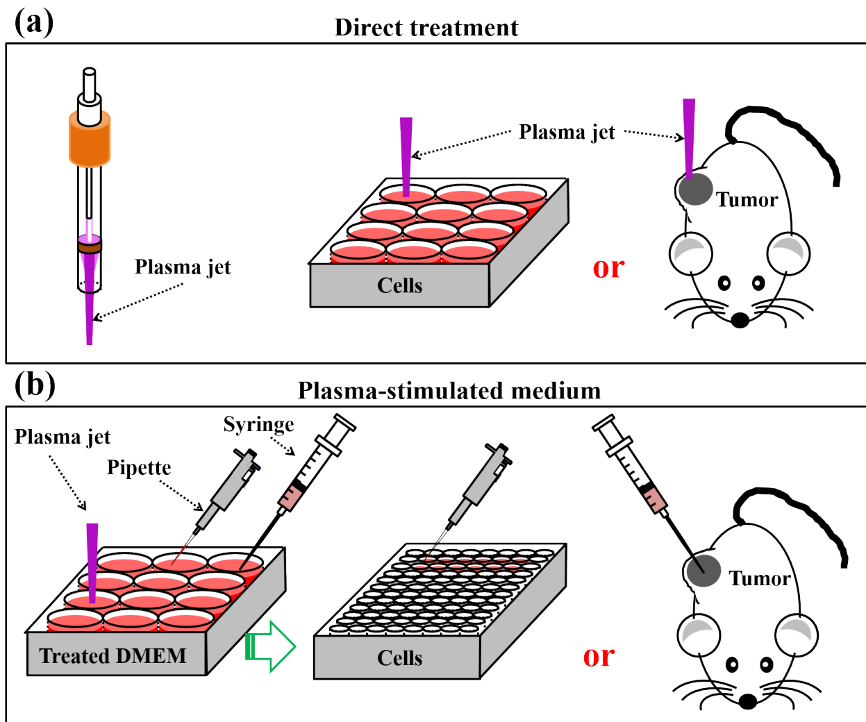
Figure 4: Two basic strategies to use CAP. a. Direct CAP treatment on cancer cells in vitro or on subcutaneous xenografted tumors in vivo . b. Indirect CAP treatment on solutions mainly medium. These PSM will be used to inhibit the growth of cancer cells seeded in multi-wells plate or the tumor tissues in mice.
